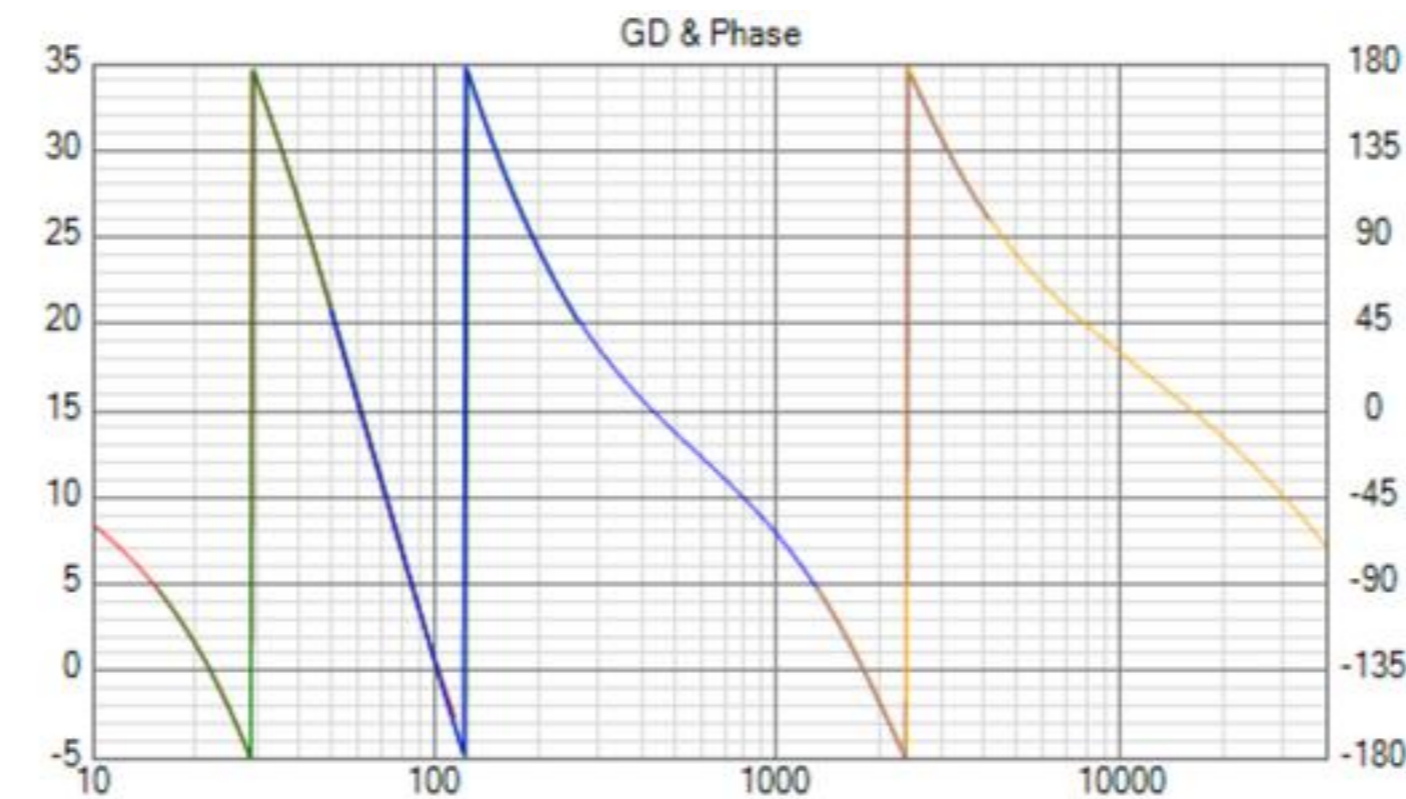
Figure 2. Phase plot of four-way system. Crossover topology used to achieve this is proprietary.
