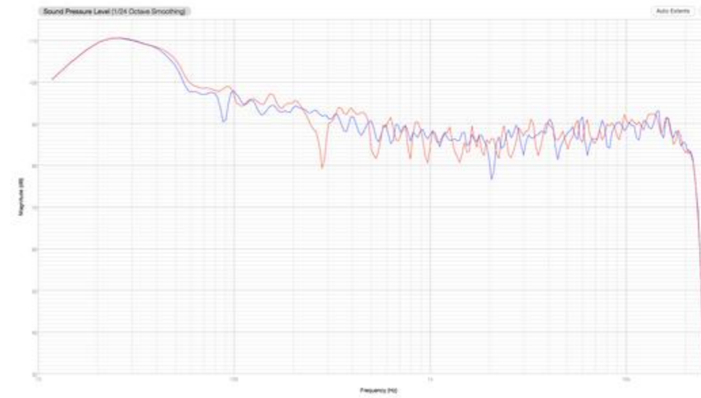
Figure 1. Frequency response of left (blue) and right (red) channels including mono subwoofer.
